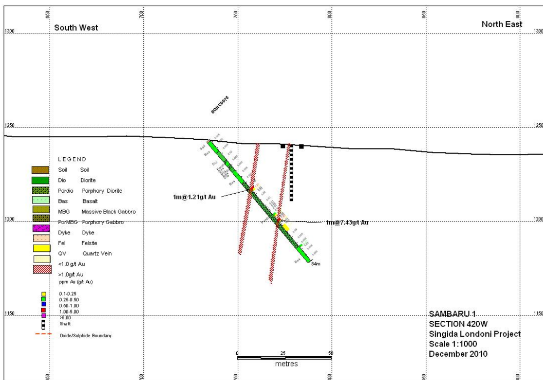
Sambaru 1-Section_420W
