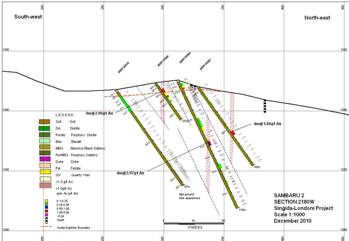
Sambaru 2-Section_2180W
