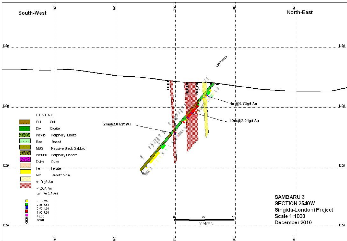
Sambaru 3-Section_2540W
