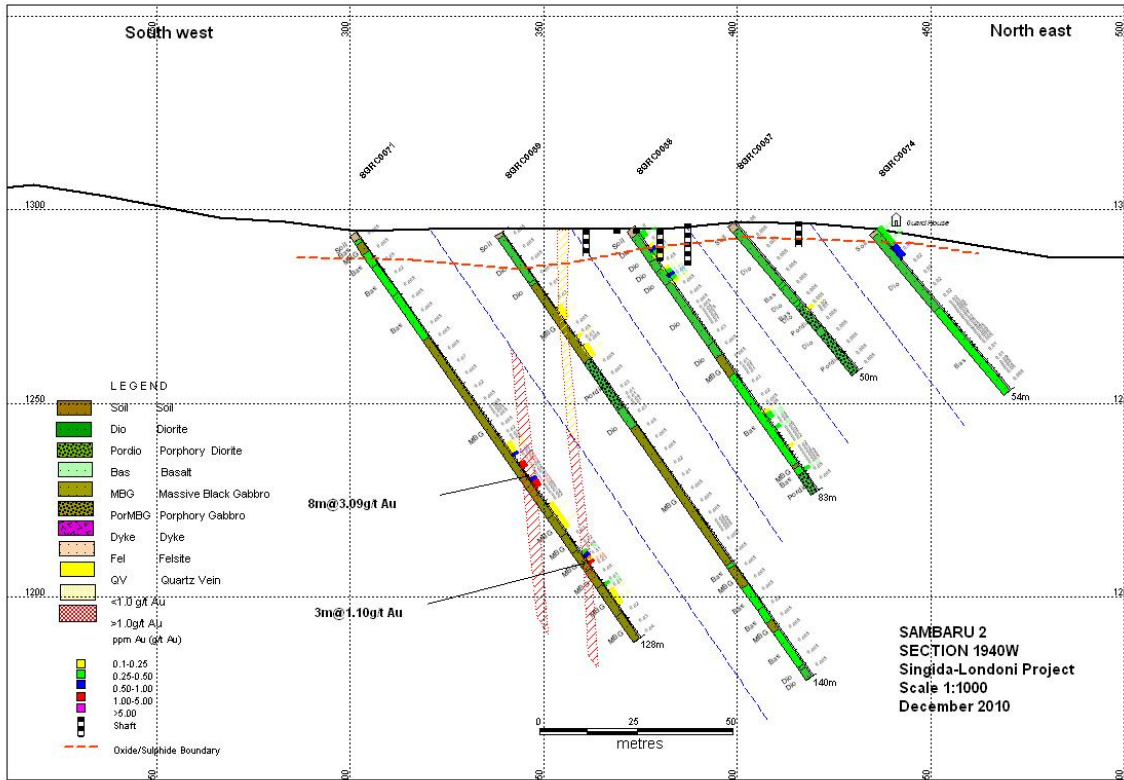
Sambaru 2-Section_1940W
