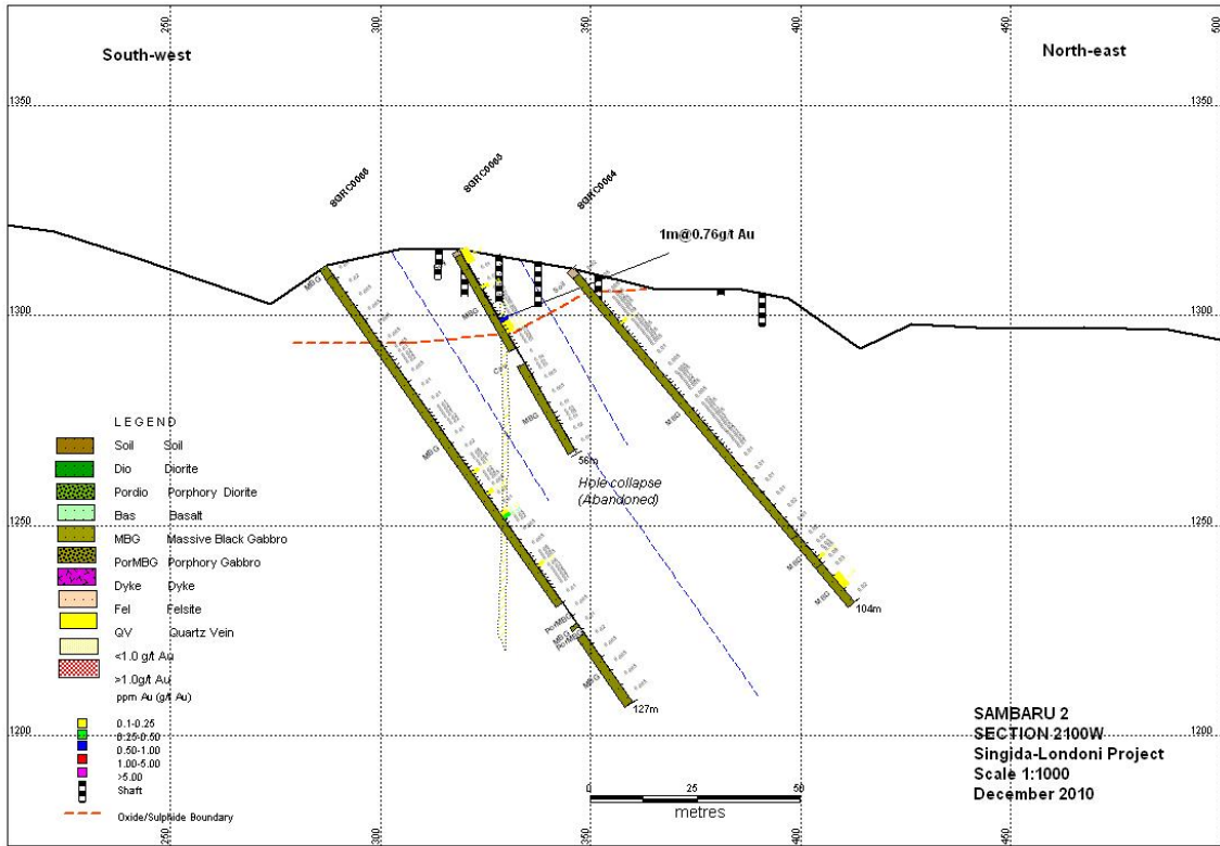
Sambaru 2-Section_2100W
