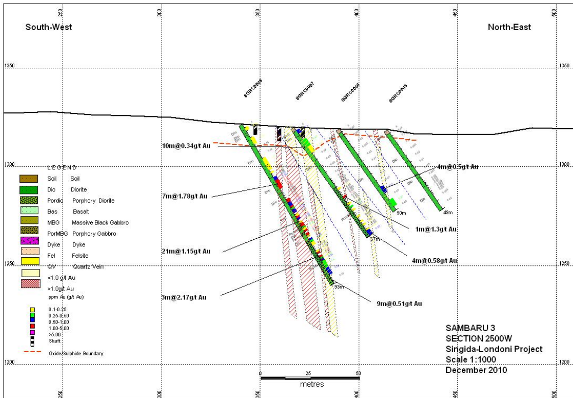
Sambaru 3-Section_2500W
