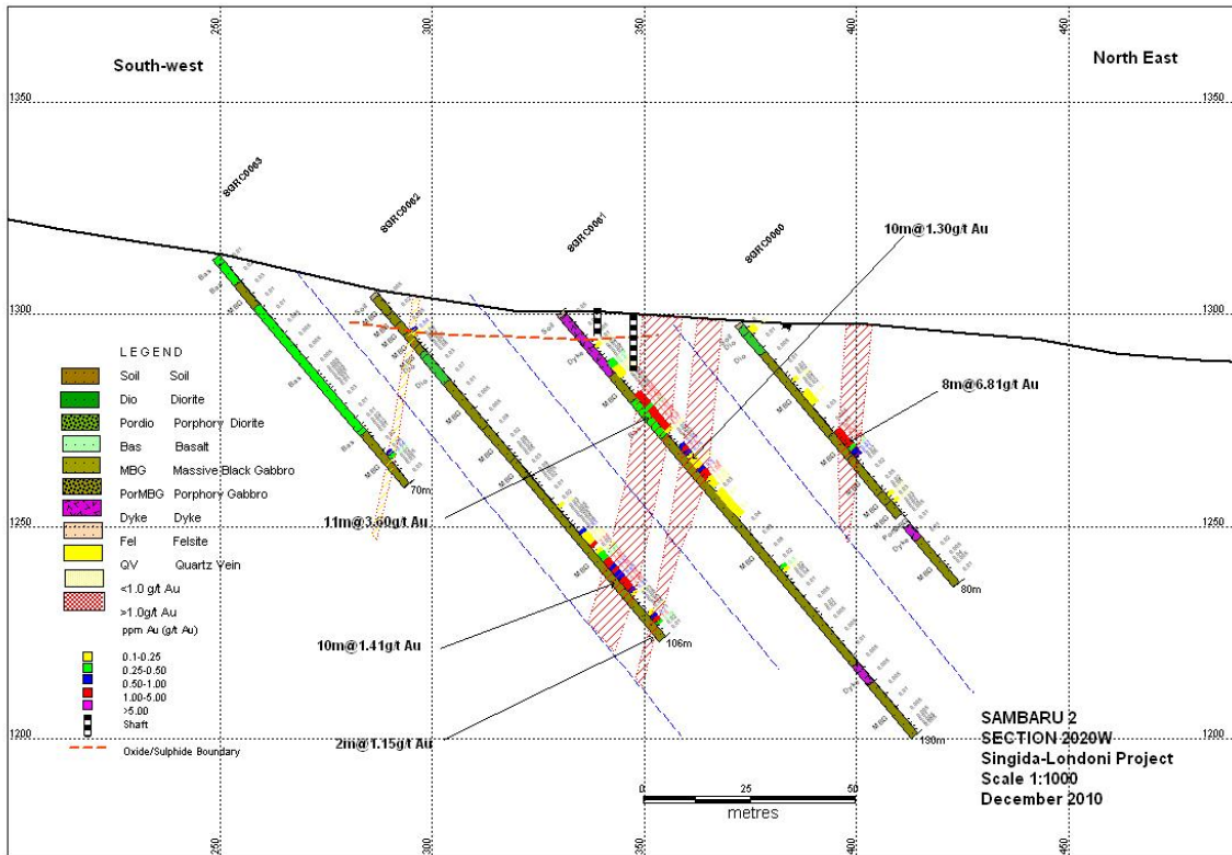
Sambaru 2-Section_2020W
