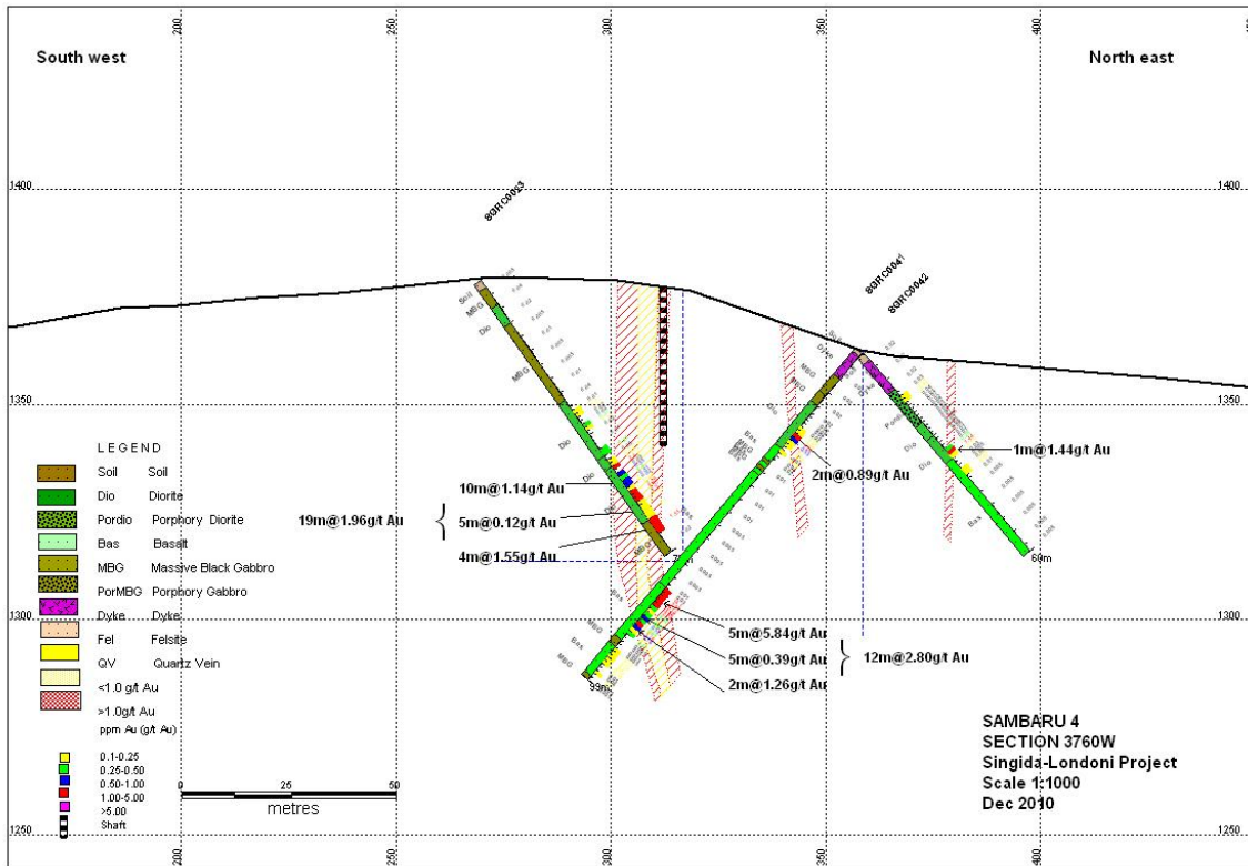
Sambaru 4-Section_3760W
