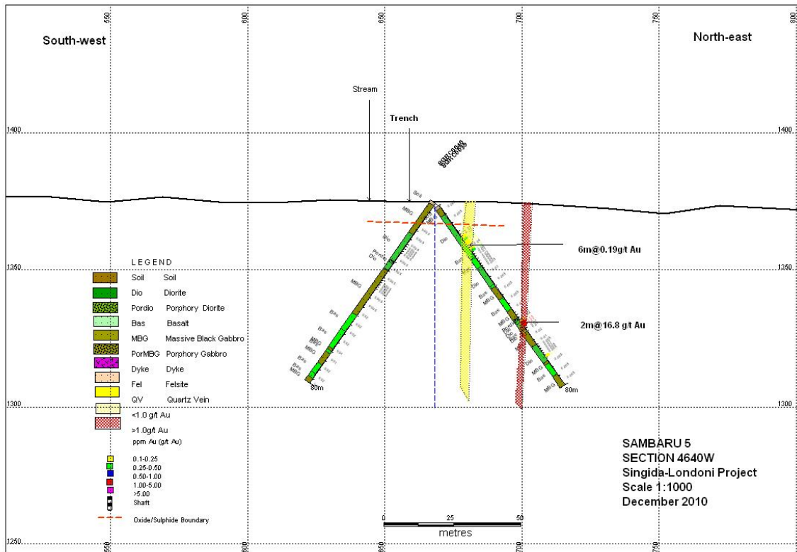
Sambaru 5-Section_4640W
