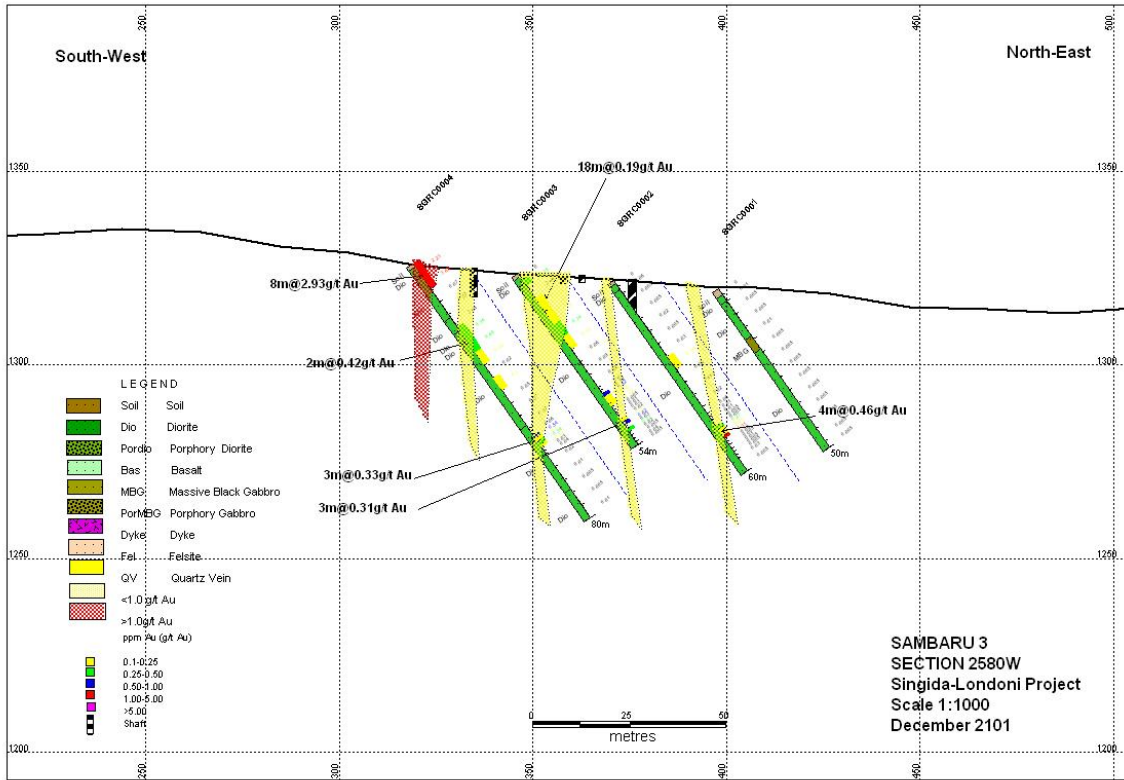
Sambaru 3-Section_2580W
